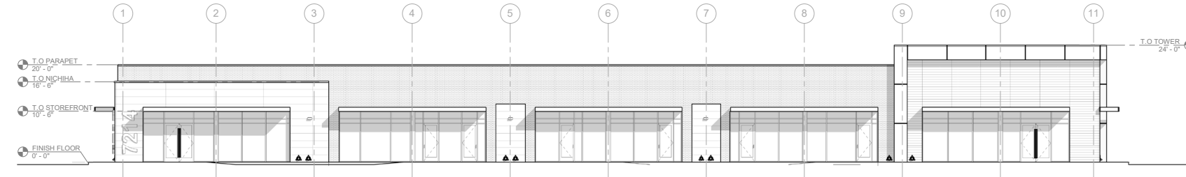
02 EXTERIOR ELEVATIONS 1/8" = 1'-0"
