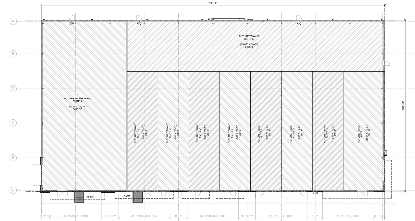
01 OVERALL FLOOR PLAN 1/8" = 1'-0"
